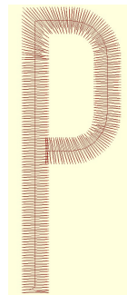
Tall Block Narrow 150 Lower P.pes 0.52x1.51 inches; 464 stitches 1 thread changes; 1 colors
